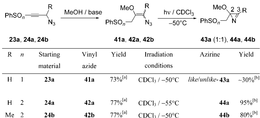
Scheme 8. [a] Yield of isolated product. [b] Yield determined by NMR.
